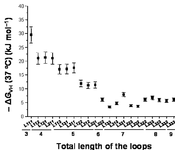
FIGURE 5: Changes in \Delta G_{\text{VH}} as a function of total loop length.
